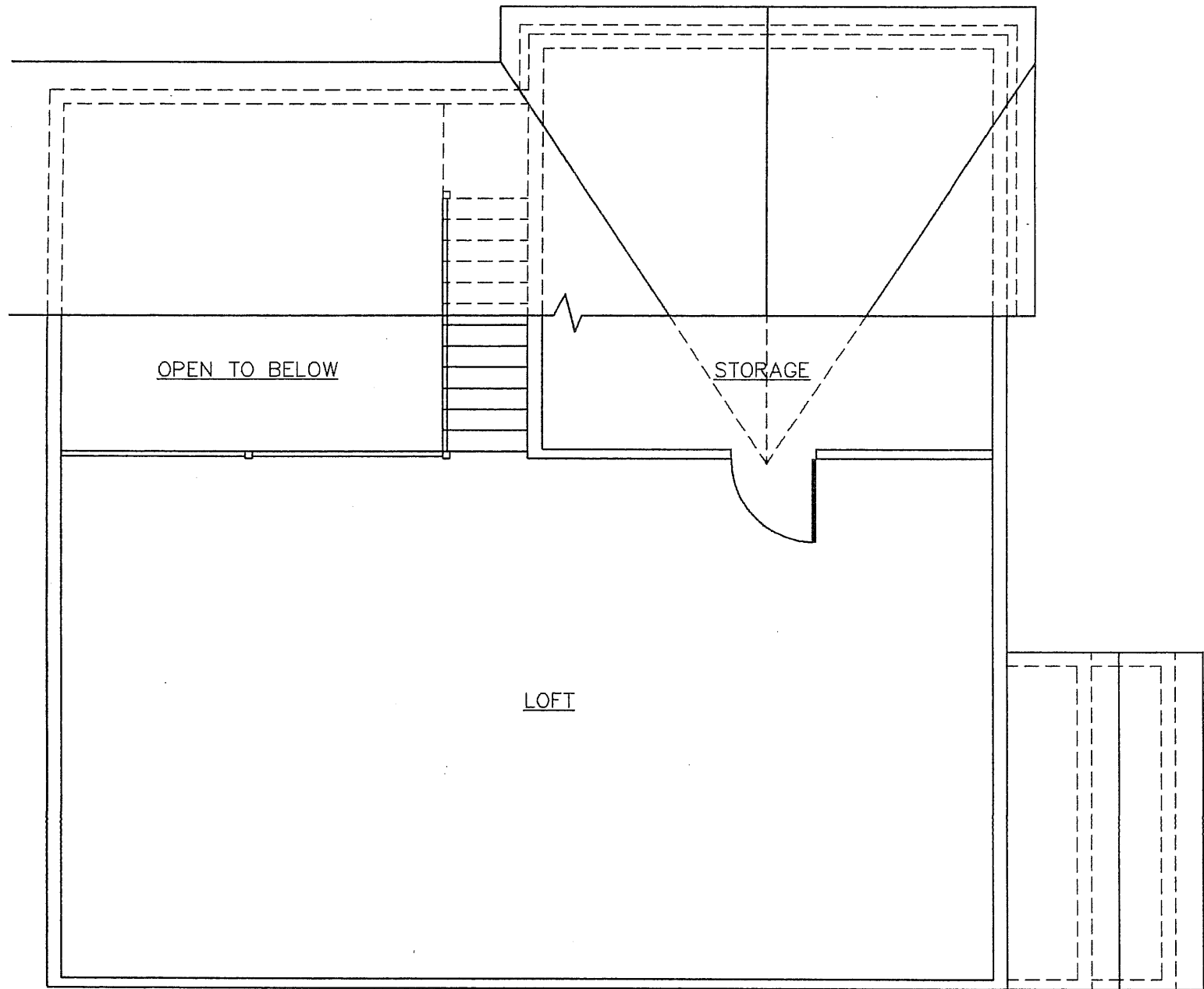
TYPE D - 1,630 SQ. FT. TWO BEDROOM TWO BATH WITH LOFT
