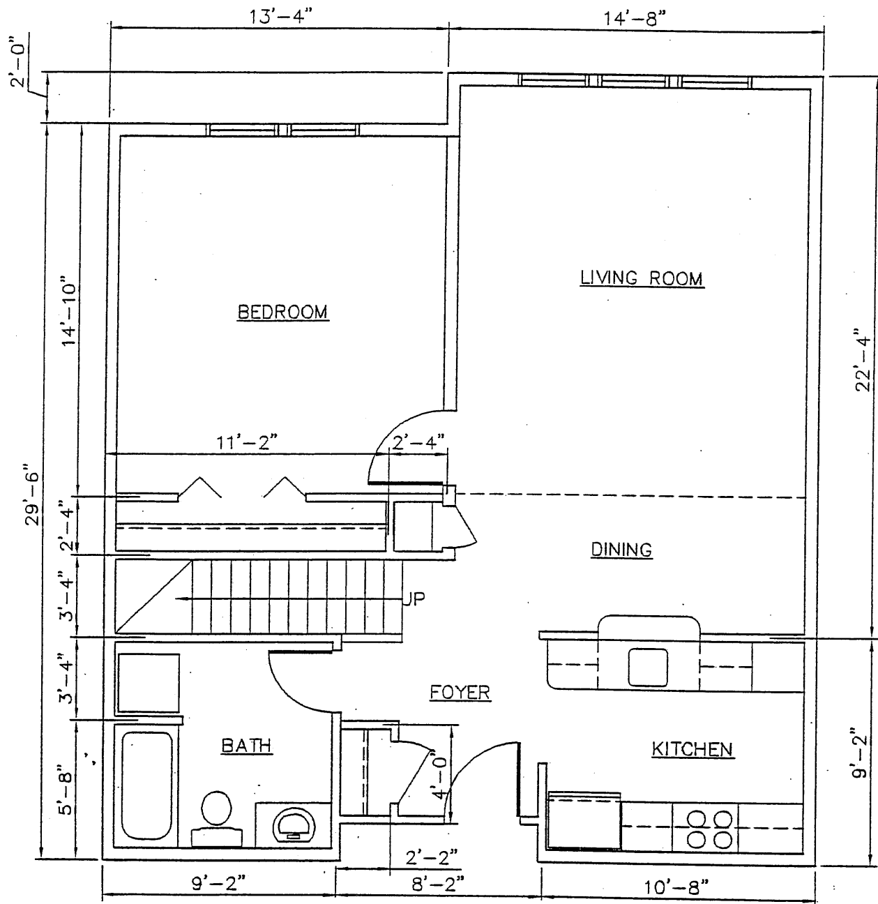
TYPE B - 1,245 SQ. FT. ONE BEDROOM WITH LOFT
