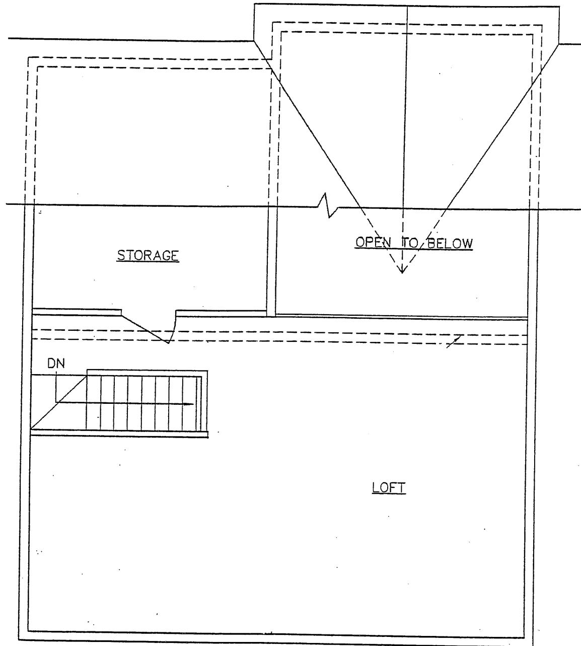
TYPE B - 1,245 SQ. FT. ONE BEDROOM WITH LOFT
